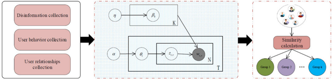
Fig. 1. Flow chart of social user groups division. The flow chart is divided into three phases. The first stage is social network attribute collection, which includes disinformation collection, user behaviour collection and user relationship collection. The second stage is social user topics distribution modelling. The meaning of each symbol is described in detail in this section. The dynamic social user groups distribution is described in stage 3. Each group represents a collection of users who propagate information about a particular topic.
