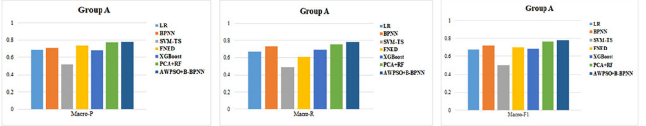
(a) Overall performance comparison with different approaches over Group A
