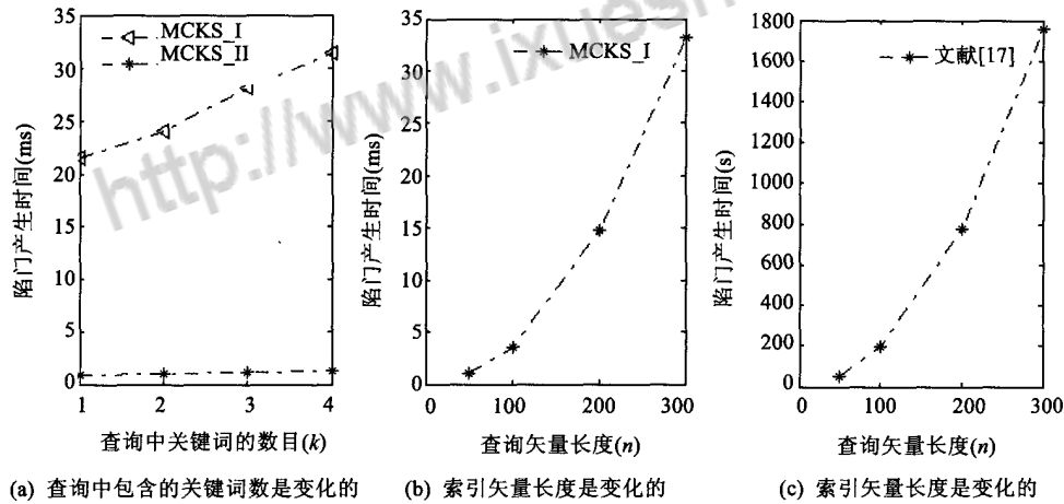
Fig.9 Trapdoor generation time
