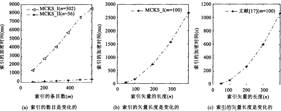
Fig.8 Comparison of the time of encrypting index vectors
