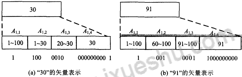
Fig.4 Vector representation of hierarchical age
