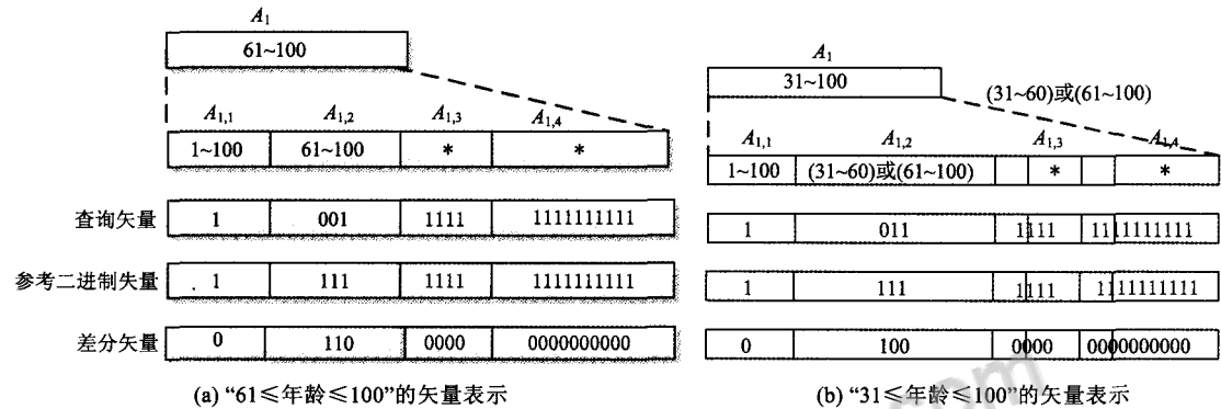
Fig.6 Vector representation of range
