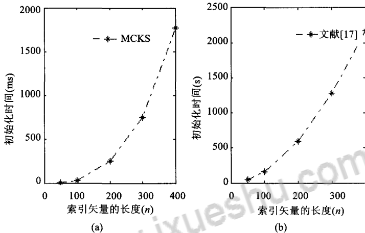
Fig.7 Relation of setup time and the length of index vectors
