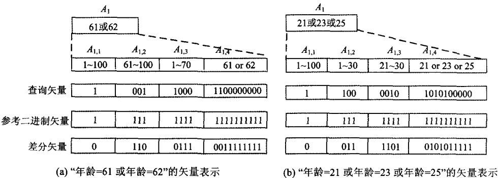
Fig.5 Vector representation of subset
