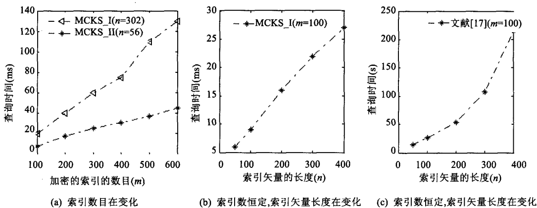
Fig.10 Query time
