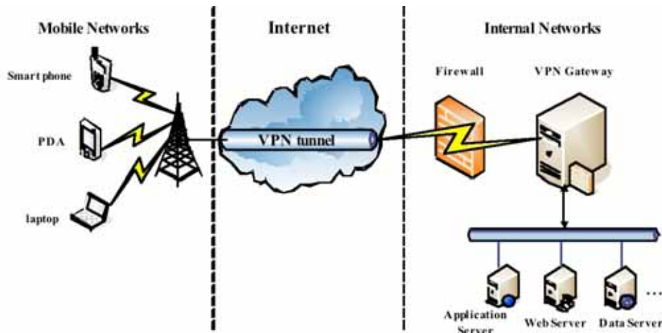
Fig. (2). Mobile VPN network topology.
