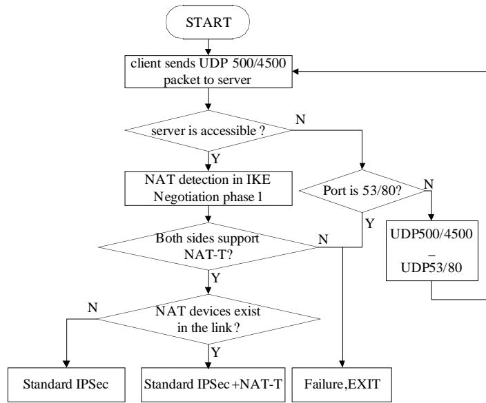
Fig. (4). Flow chart of adaptive dial-up policy.
