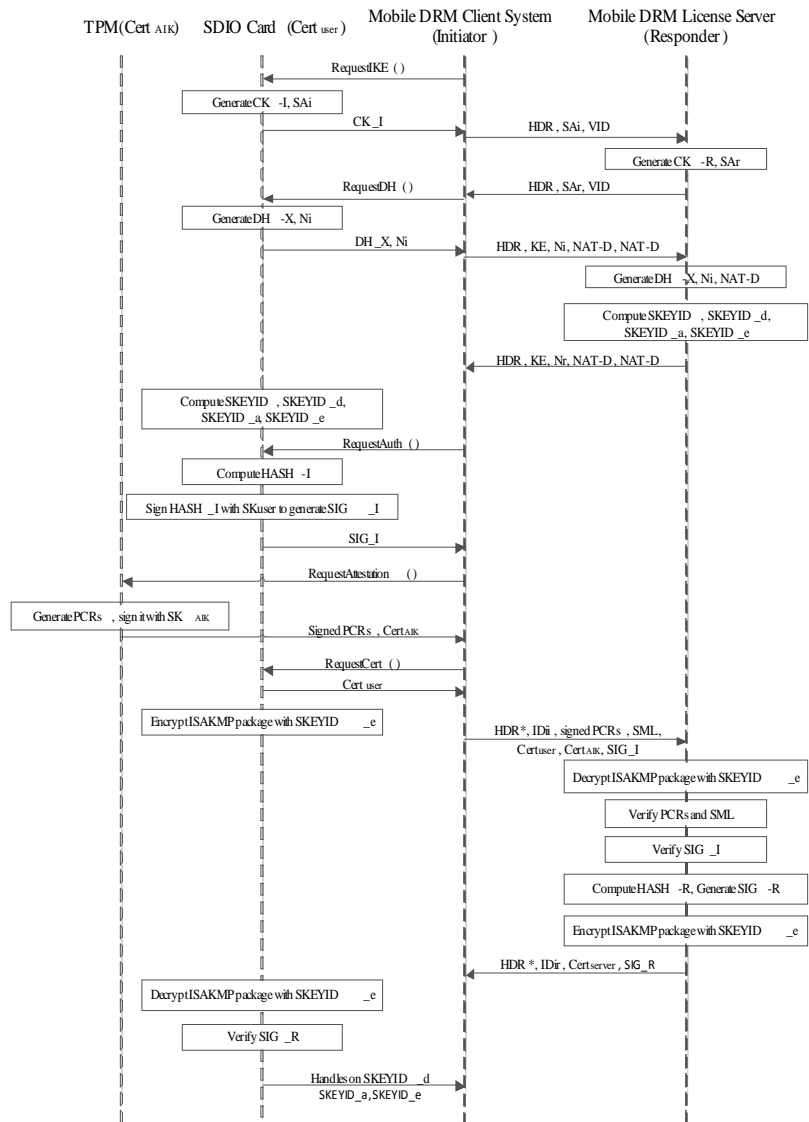
Fig. (5). Flow chart of remote attestation extended IKE.
